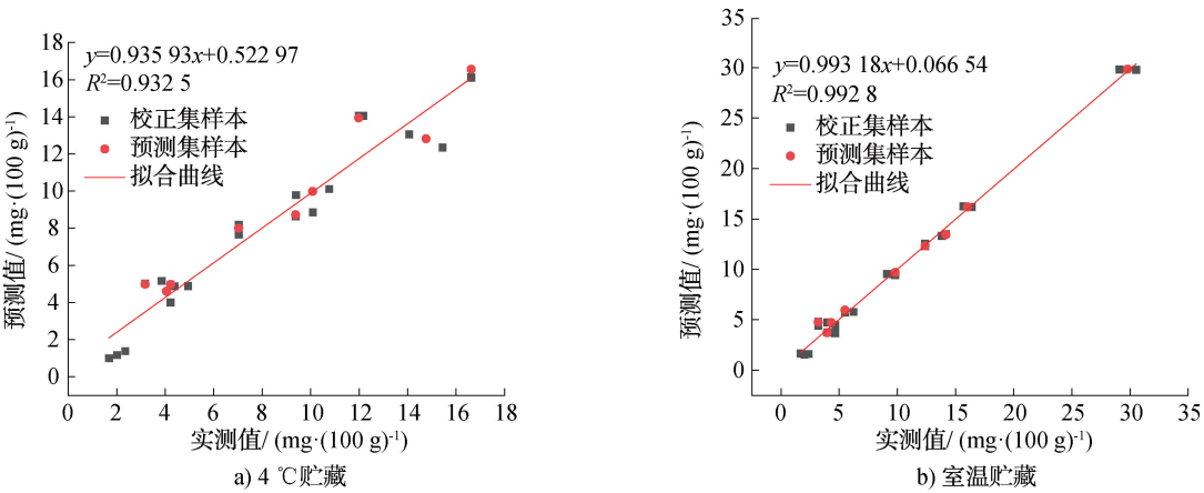
图 6 Stepwise-MLR 模型预测结果 Fig. 6 Prediction results of Stepwise-MLR models
