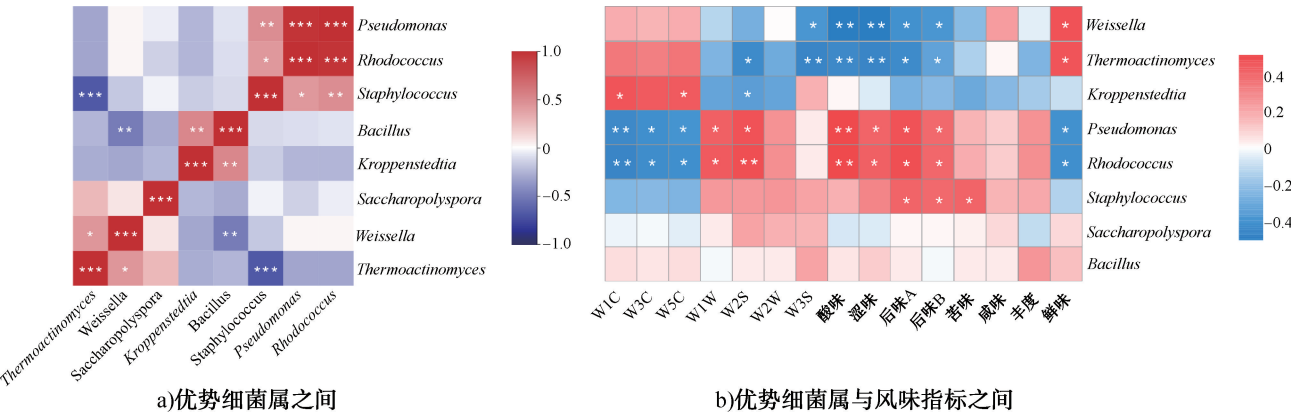
图 6 不同颜色高温大曲中优势细菌属之间及优势细菌属与风味指标之间的 Spearman 相关性分析结果 Fig. 6 Results of Spearman correlation analysis between dominant bacterial genera and flavor indicators of different colored high-temperature Daqu
