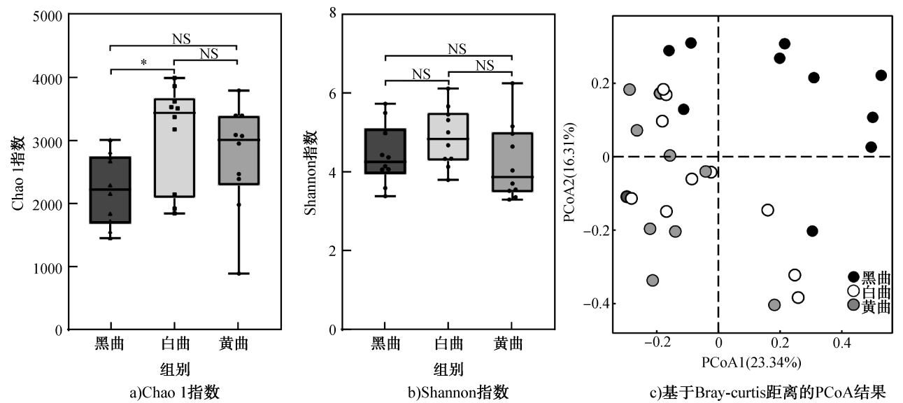
图 3 不同颜色高温大曲细菌的 Chao1 指数、Shannon 指数和基于 Bray-curtis 距离的 PCoA 结果 Fig. 3 Bacterial Chao1 index, Shannon index, and PCoA results based on Bray-Curtis distance of different colored high-temperature Daqu
