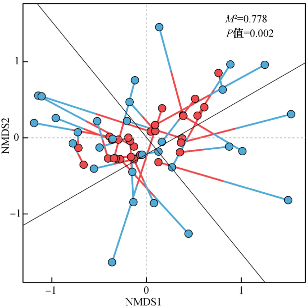
图 5 不同颜色高温大曲中优势细菌属与风味品质之间的普氏分析结果 Fig. 5 Results of the Procrustes analysis between the dominant bacterial genera and flavor indicators of different colored high-temperature Daqu
